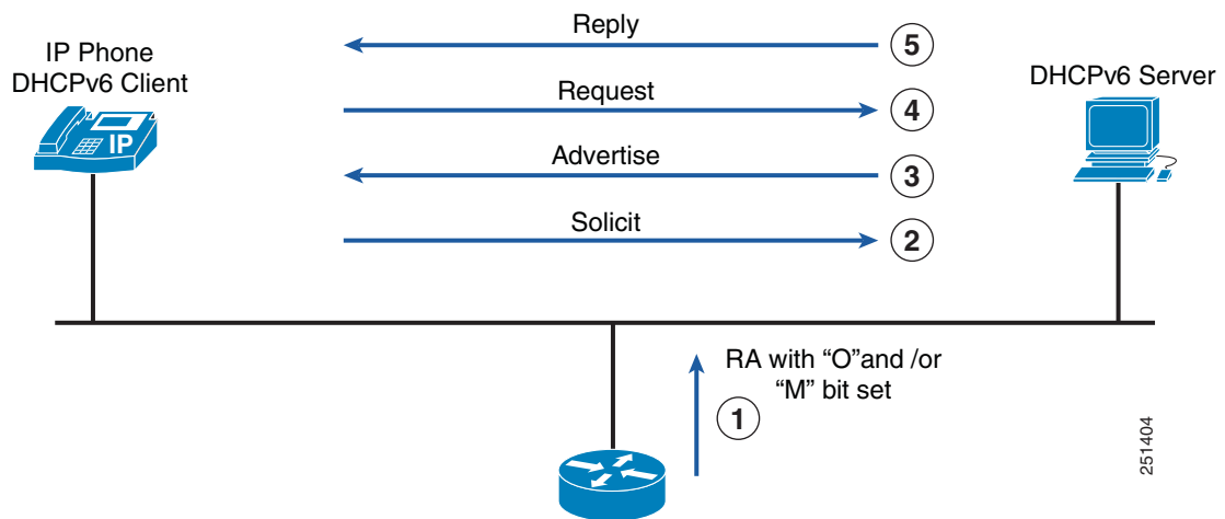
Figure 2-8 IPv6 DHCP operation
