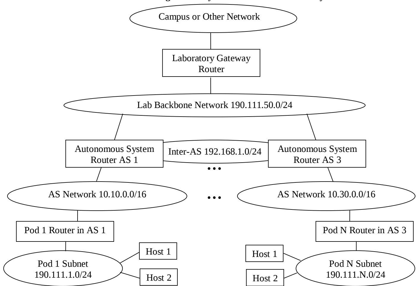
Figure Lab-4. Logical Diagram.
